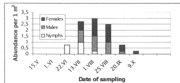
Fig. 5: Seasonal dynamics of Oecanthus pellucens at CV site in 2000
