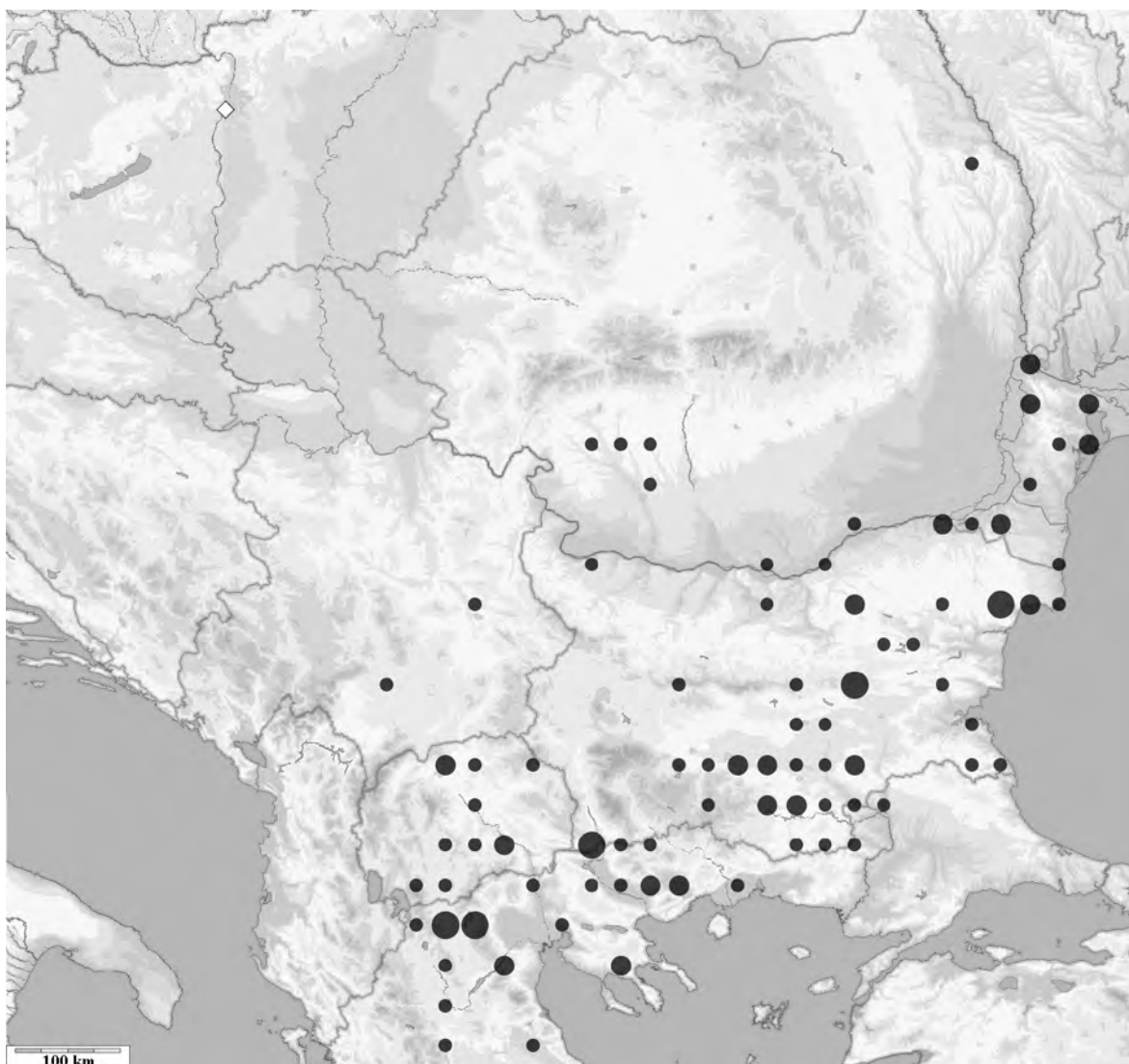
Fig. 6: Distribution map (performed with Flauna © E. Polidori, 2002-08).
